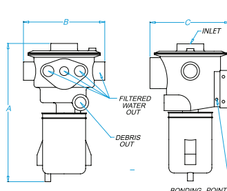
970-1500 DIMENSIONS
