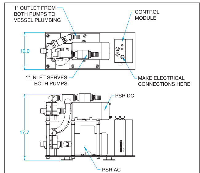
PARALLELAGON™ VERTICAL DIMENSIONS
