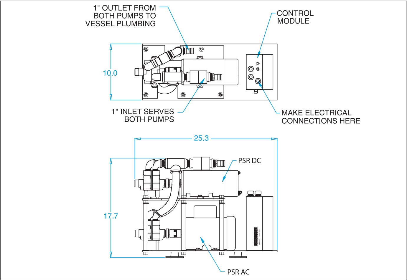
PARV DIMENSIONS
