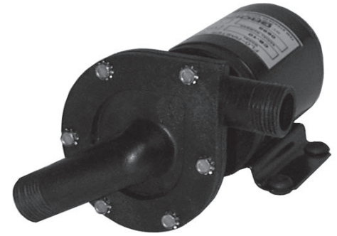
CB-10 Inlet and Outlet are for garden hose connections or for 1" ID hose
