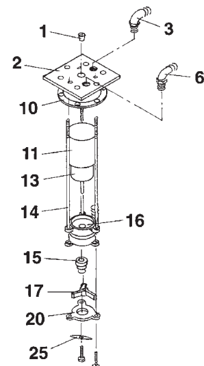
Sample Installation shows 155-series Macerator Pump and related components
